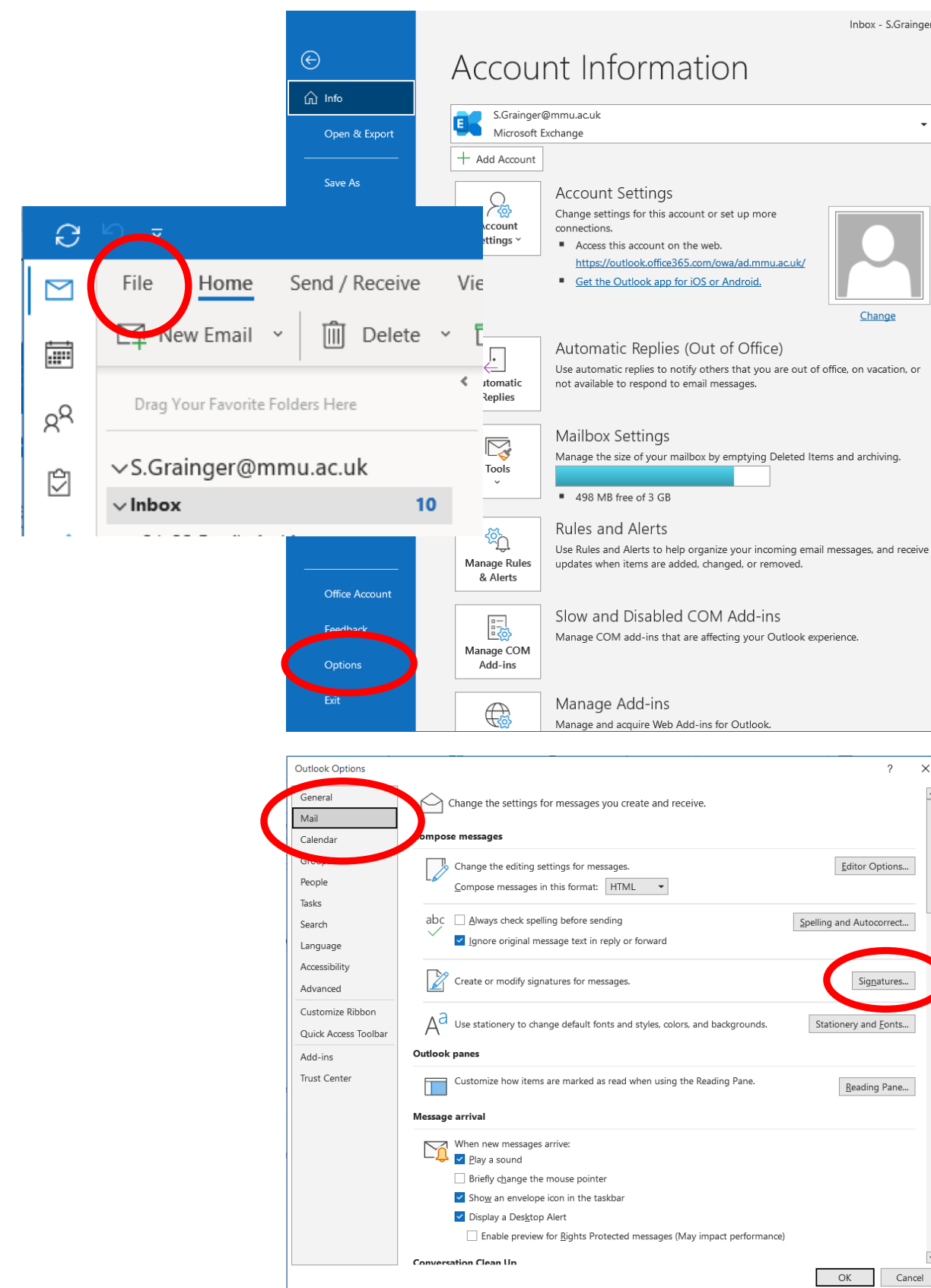
Desktop App
