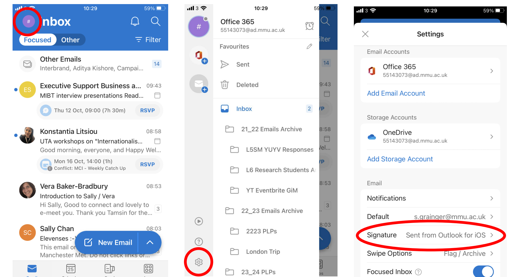
Mobile App
